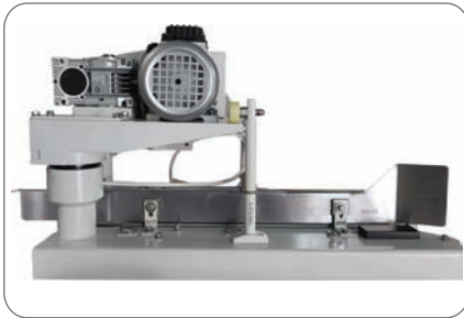
Automatic Infeed
